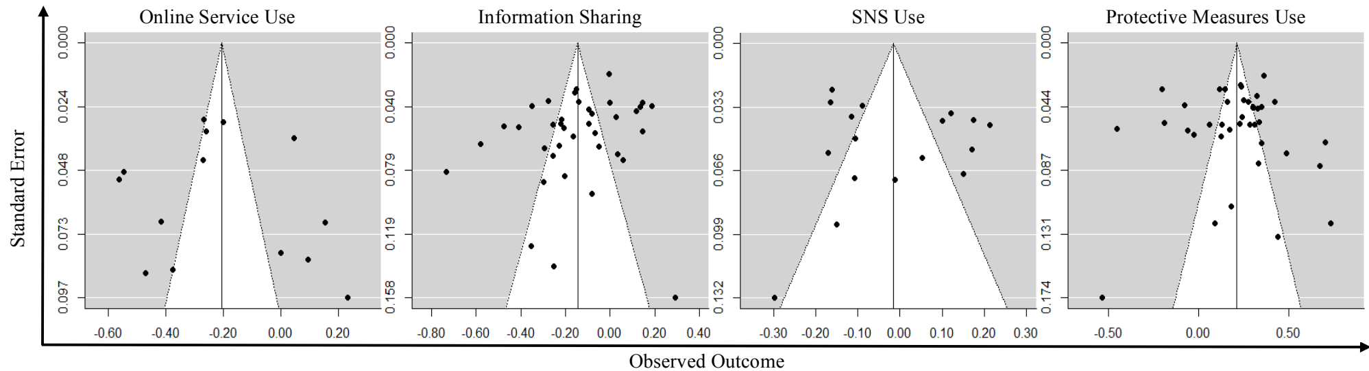
Supplementary Figure 16. Funnel Plots of the Meta-Analyses Investigating the Associations between Privacy Concern and Online Service Use (Non-SNS), Information Sharing, SNS Use and Protective Measures Use Using Trim-Fill Procedure
